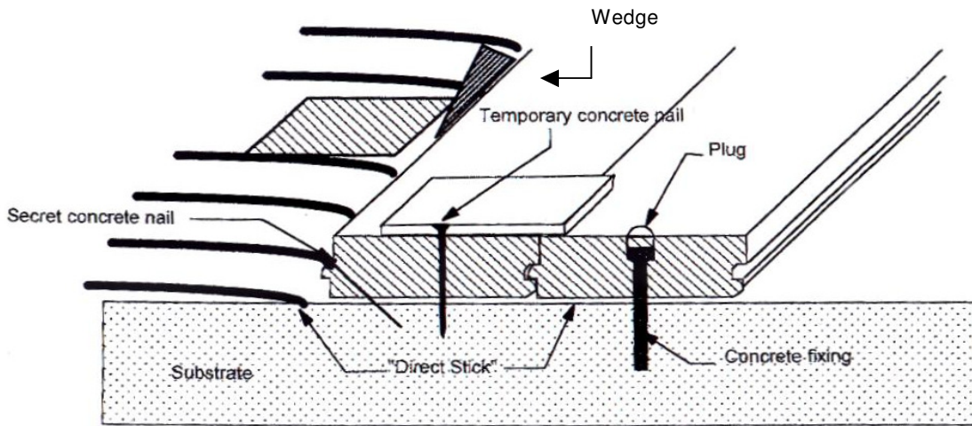
Some systems of holding timber to concrete while the glue sets
