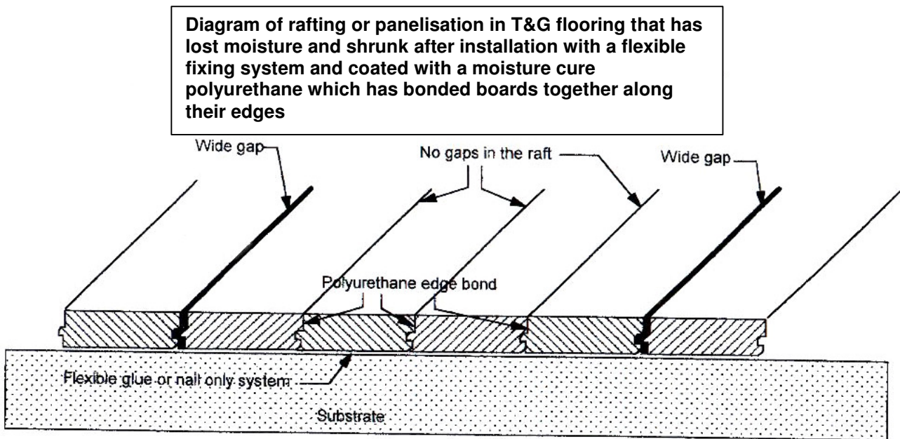
Diagram C3. Rafting (panelisation) in strip flooring installed with a flexible adhesive system
