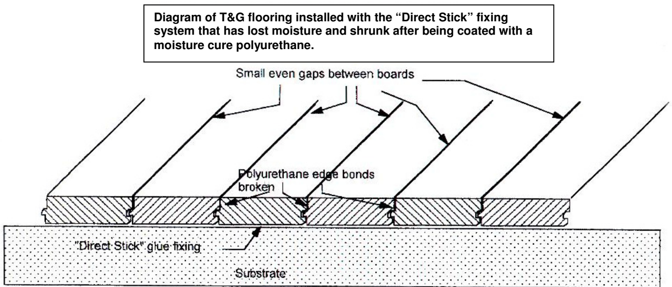
Diagram 4. LIQUID NAILS DIRECT STICK laid onto a continuous substrate resists the forces that cause rafting (panelisation).
